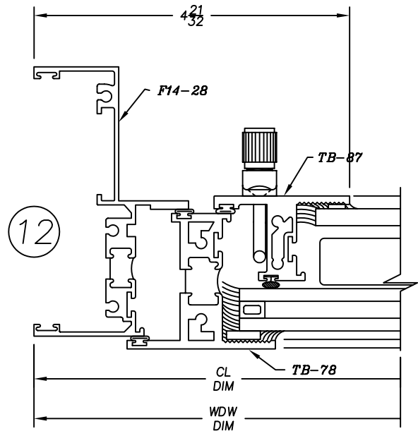
Right Hand Out-Swing Casement
