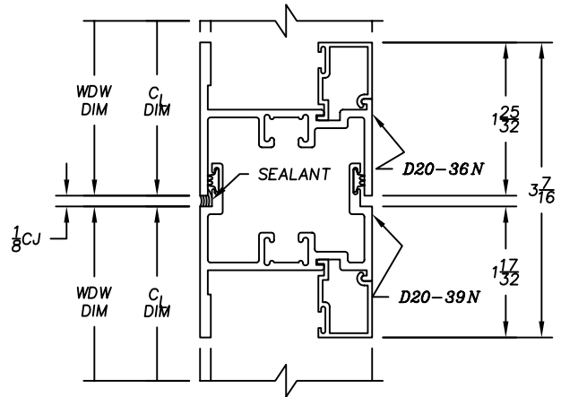
2200 SERIES - HORIZONTAL STACK D20-36N / D9-39N (VENTS USE SAME EXTRUSION)
