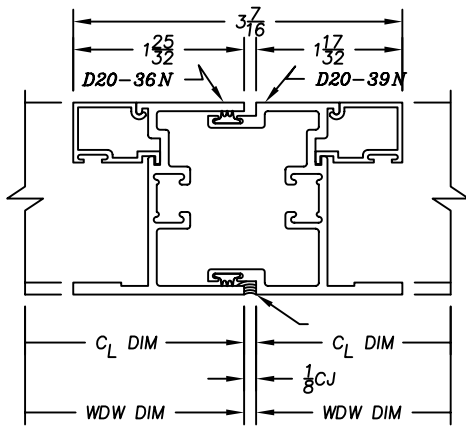
2200 SERIES - VERTICAL STACK D20-36N / D9-39N (VENTS USE SAME EXTRUSION)
