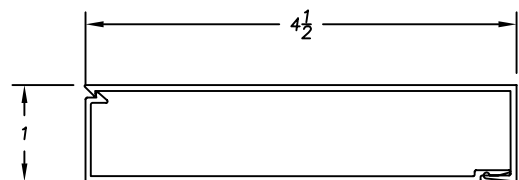
D8-243 SNAP COVER D8-244 BASE CLIP
