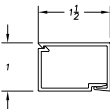
D8-220 SNAP COVER D8-221 BASE CLIP
