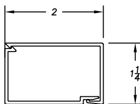
D8-202 SNAP COVER D8-203 BASE CLIP
