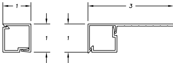
D8-229 SNAP COVER D8-226 BASE CLIP
