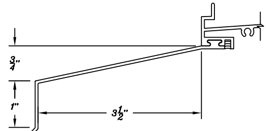
D33-105 3 1/2" SILL EXTENSION
