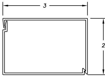
D8-271 SNAP COVER D8-272 BASE CLIP
