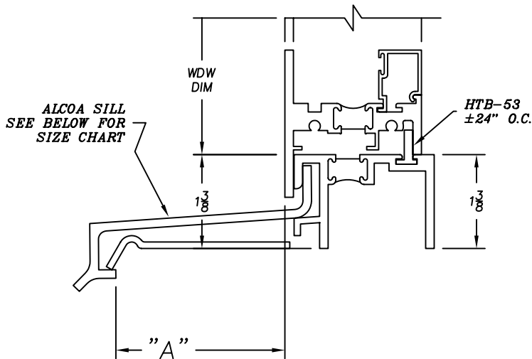
TB-54 SILL STARTER For Use Only With Alcoa Sills For All 2" Windows
