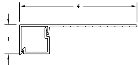
D8-225 SNAP COVER D8-226 BASE CLIP
