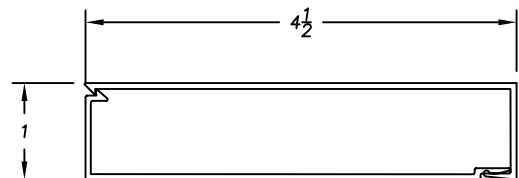
D8-243 SNAP COVER D8-244 BASE CLIP
