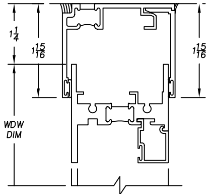
TB-25 SUB-FRAME & D11-148 CLOSURE PLATE FOR ALL 2" THERMAL WINDOWS
