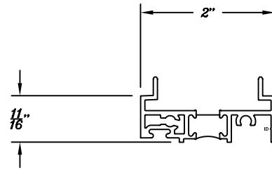
TB-102 SUB-SILL For All 2" Thermal Windows
