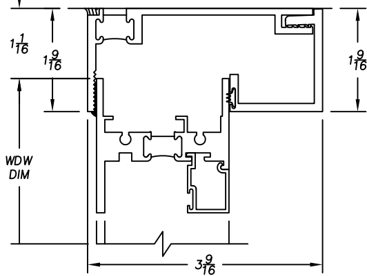
D17-25 SUB-FRAME & TB-130 CLOSURE PLATE FOR ALL 2" THERMAL WINDOWS
