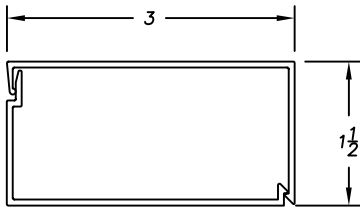
D8-169 SNAP COVER D8-170 BASE CLIP
