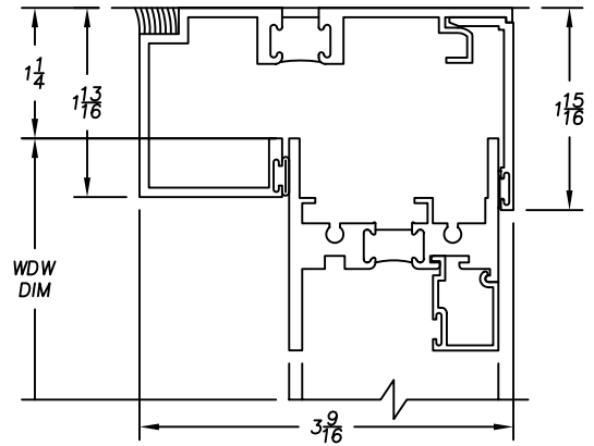
TB-225 SUB-FRAME & D11-148 CLOSURE PLATE FOR ALL 2" THERMAL WINDOWS
