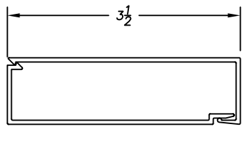
D8-205 SNAP COVER D8-206 BASE CLIP
