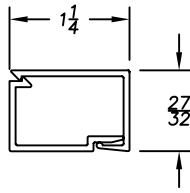
D8-179 SNAP COVER D8-180 BASE CLIP
