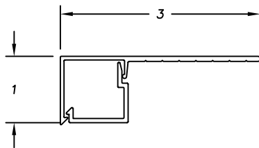
D8-227 SNAP COVER D8-226 BASE CLIP
