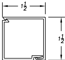
D8-209 SNAP COVER D8-210 BASE CLIP
