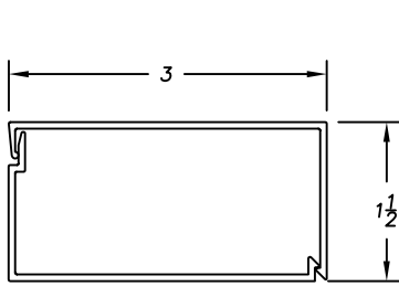
D8-169 SNAP COVER D8-170 BASE CLIP
