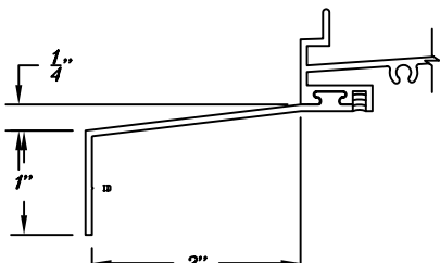
D33-108 2" SILL EXTENSION
