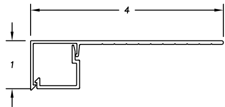
D8-225 SNAP COVER D8-226 BASE CLIP
