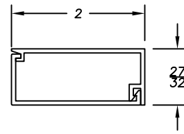
D8-173 SNAP COVER D8-174 BASE CLIP
