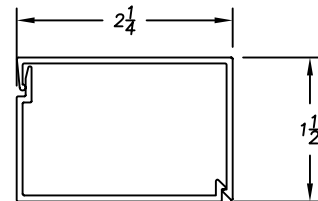
D8-171 SNAP COVER D8-172 BASE CLIP
