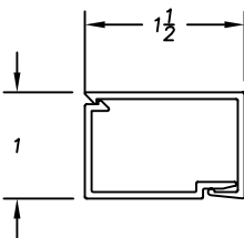
D8-220 SNAP COVER D8-221 BASE CLIP
