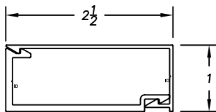
D8-233 SNAP COVER D8-232 BASE CLIP
