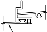
SILL EXTENSION
