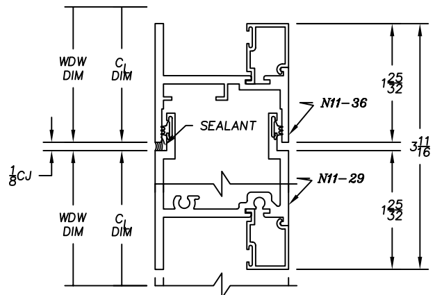
1100 SERIES – HORIZONTAL STACK N11-36 / N11-29 (VENTS USE SAME EXTRUSION)
