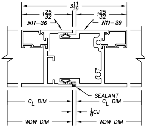
1100 SERIES – VERTICAL STACK N11-36 / N11-29 (VENTS USE SAME EXTRUSION)
