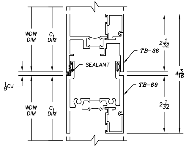
1150 SERIES – HORIZONTAL STACK TB-36 / TB-69 (VENTS USE SAME EXTRUSION)
