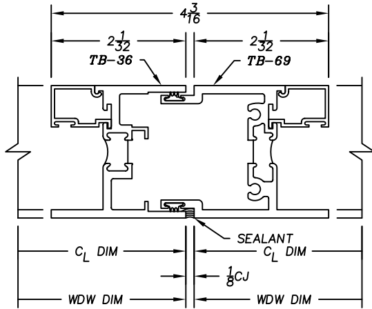
1150 SERIES – VERTICAL STACK TB-36 / TB-69 (VENTS USE SAME EXTRUSION)
