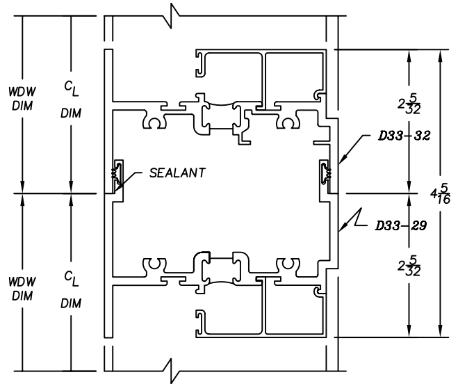
3350 SERIES - HORIZONTAL STACK D33-32 / D33-29
