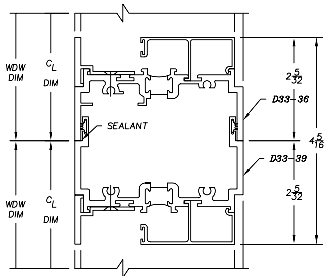
3350 SERIES - HORIZONTAL STACK D33-36 / D33-39
