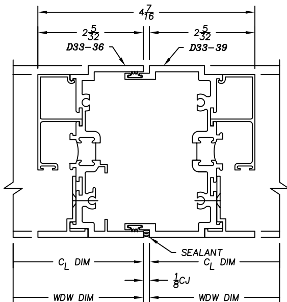
3350 SERIES - VERTICAL STACK D33-36 / D33-39
