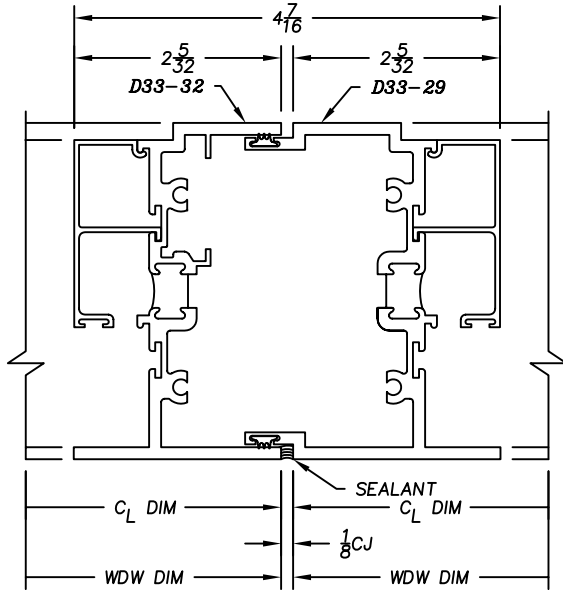
3350 SERIES - VERTICAL STACK D33-32 / D33-29
