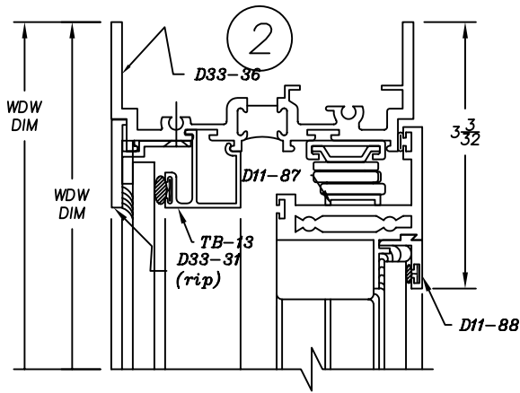
Fixed/Right Hand Out-Swing Casement
