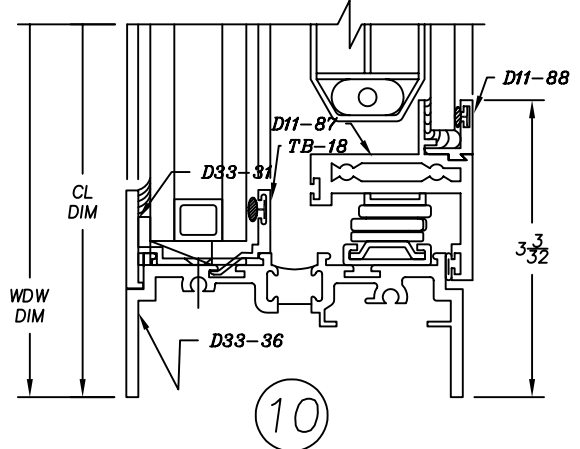
Fixed/Right Hand Out-Swing Casement
