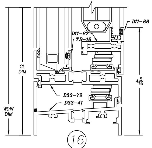
Fixed/Right Hand In-Swing Casement
