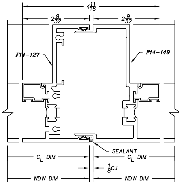
1450H SERIES - VERTICAL STACK F14-127 / F14-149
