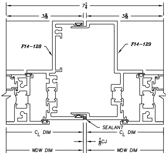
1450H SERIES - VERTICAL STACK F14-128 / F14-129
