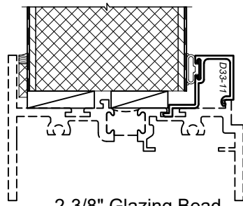
2-3/8" Glazing Bead D33-11
