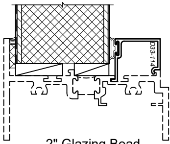
2" Glazing Bead D33-114
